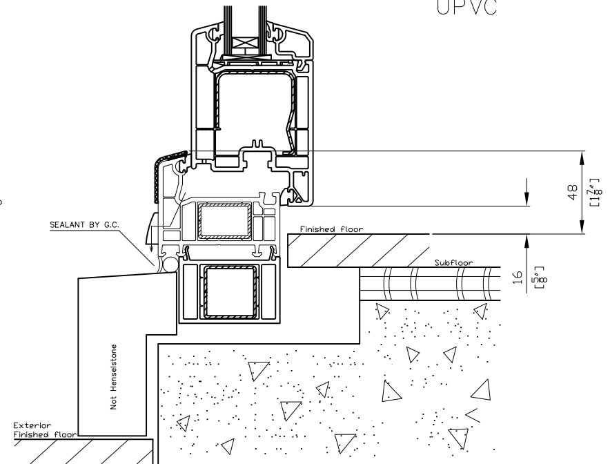
inswing UPVC
