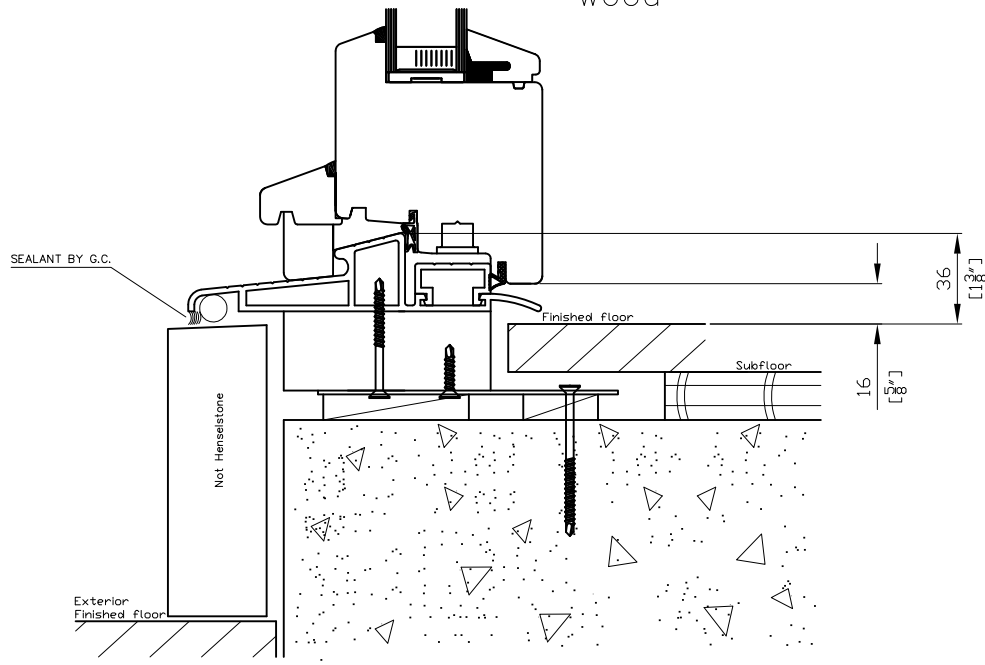
inswing wood
